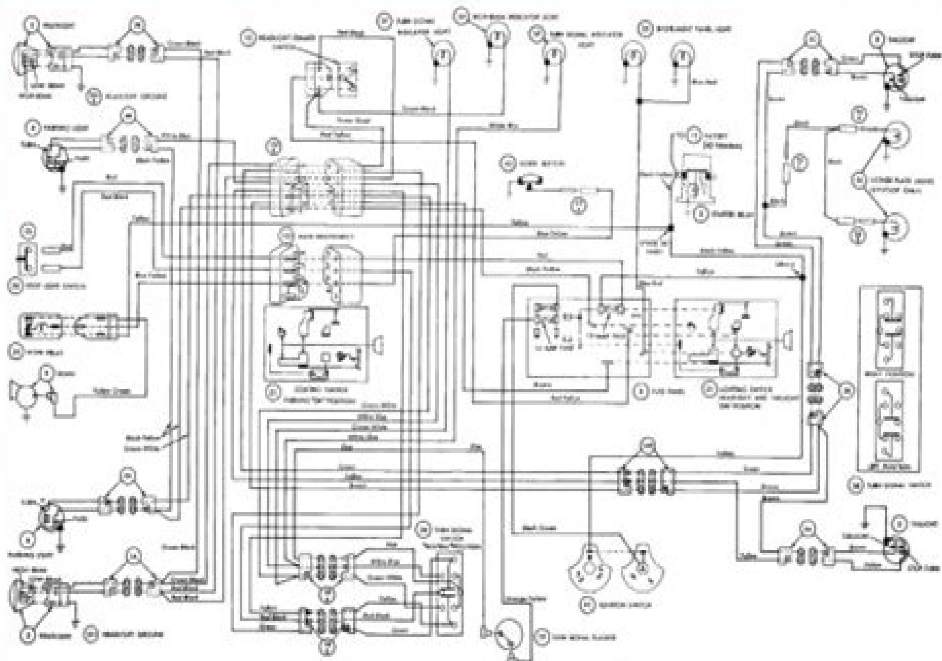
1964 F-100 THRU F-750 SERIES TRUCKS EXTERIOR LIGHTING, TURN SIGNALS AND HORN SCHEMATIC
