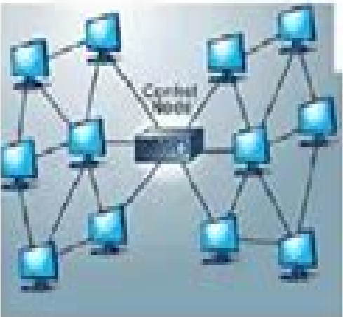
Parallel Processing
