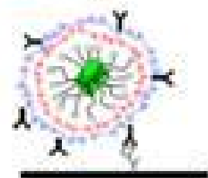
Immunoassay
