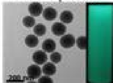
FL nanoparticle
