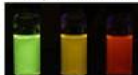
Morphochromism
