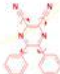
Conformation study
