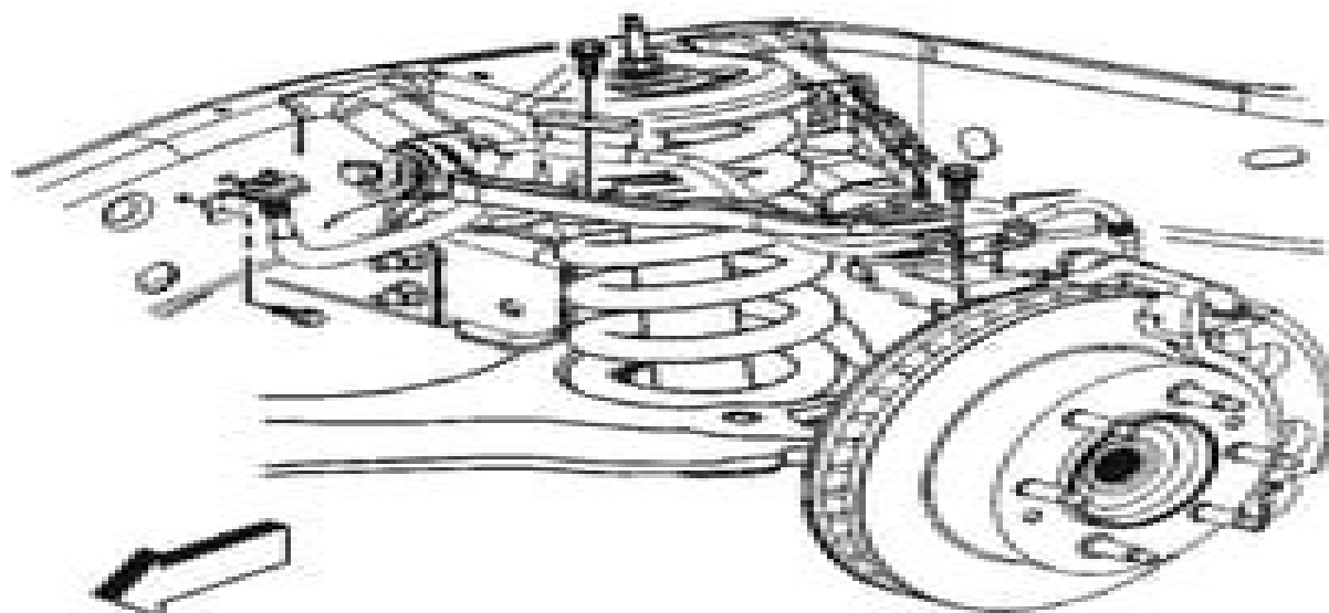
Fig. 17: View Of Retaining Bolts For Brake Hose And Wheel Speed Sensor Brackets
