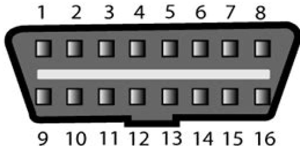
J1962 Type A
