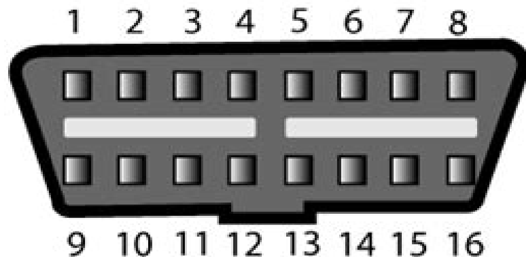
J1962 Type B
