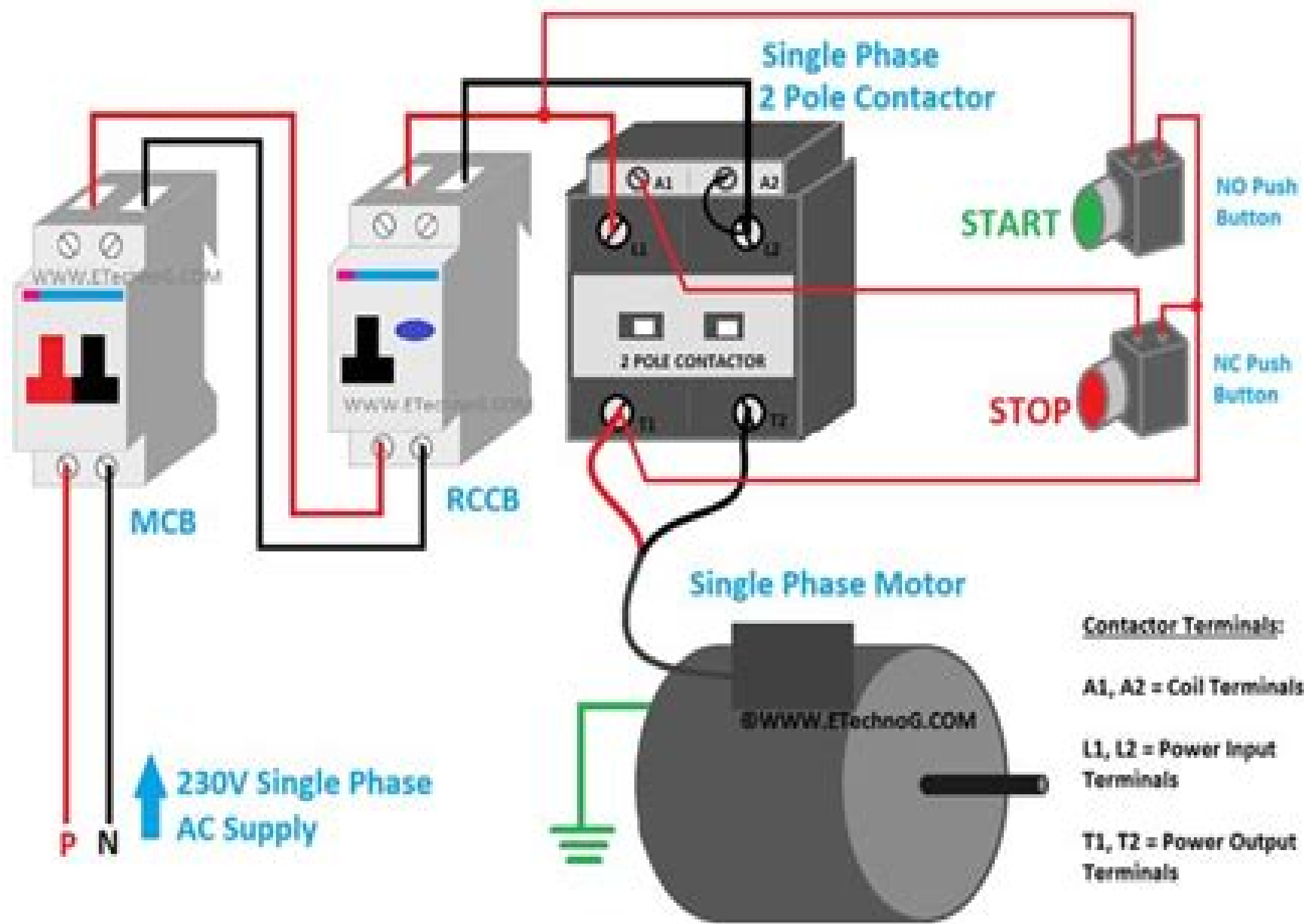
Figure.01: Single Phase 2 Pole Contactor Wiring Diagram & Connection Procedure
