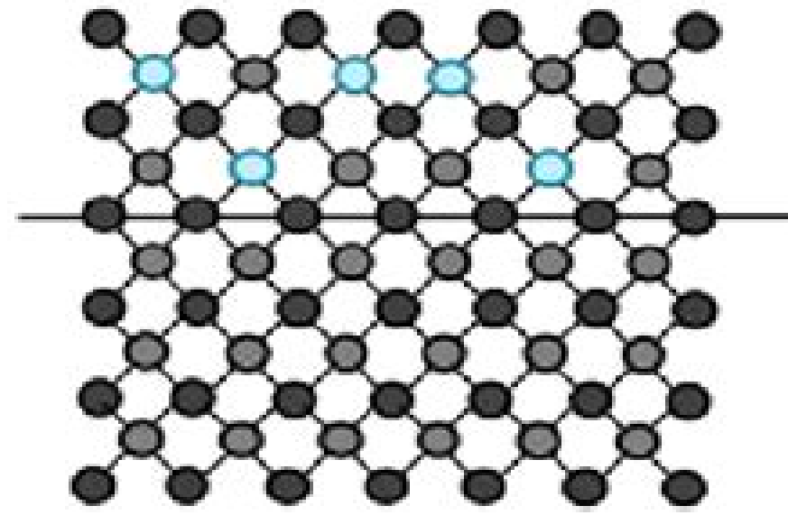
Surface Co-Precipitation
