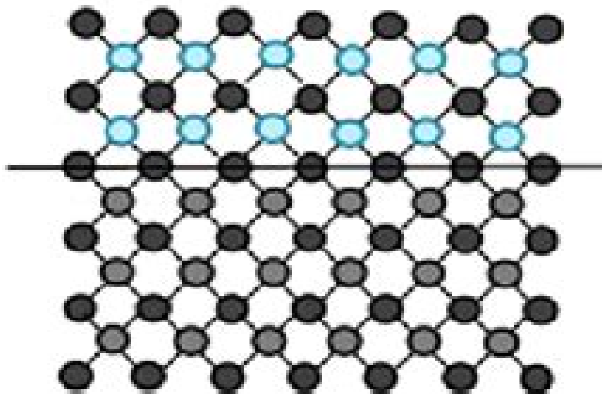
Surface Precipitation
