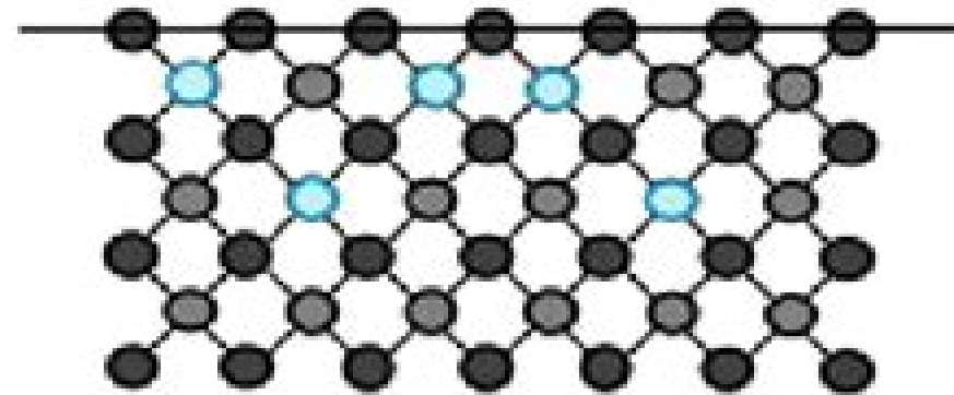
Surface Co-Precipitation
