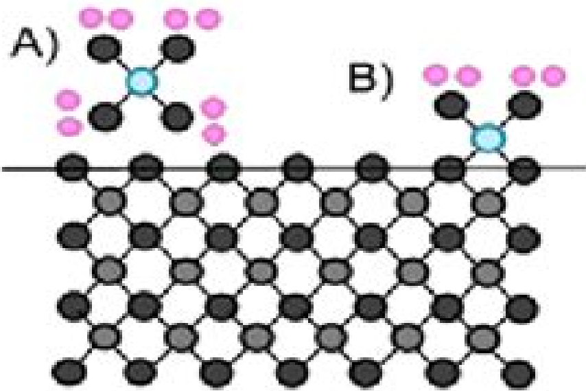
Adsorption
