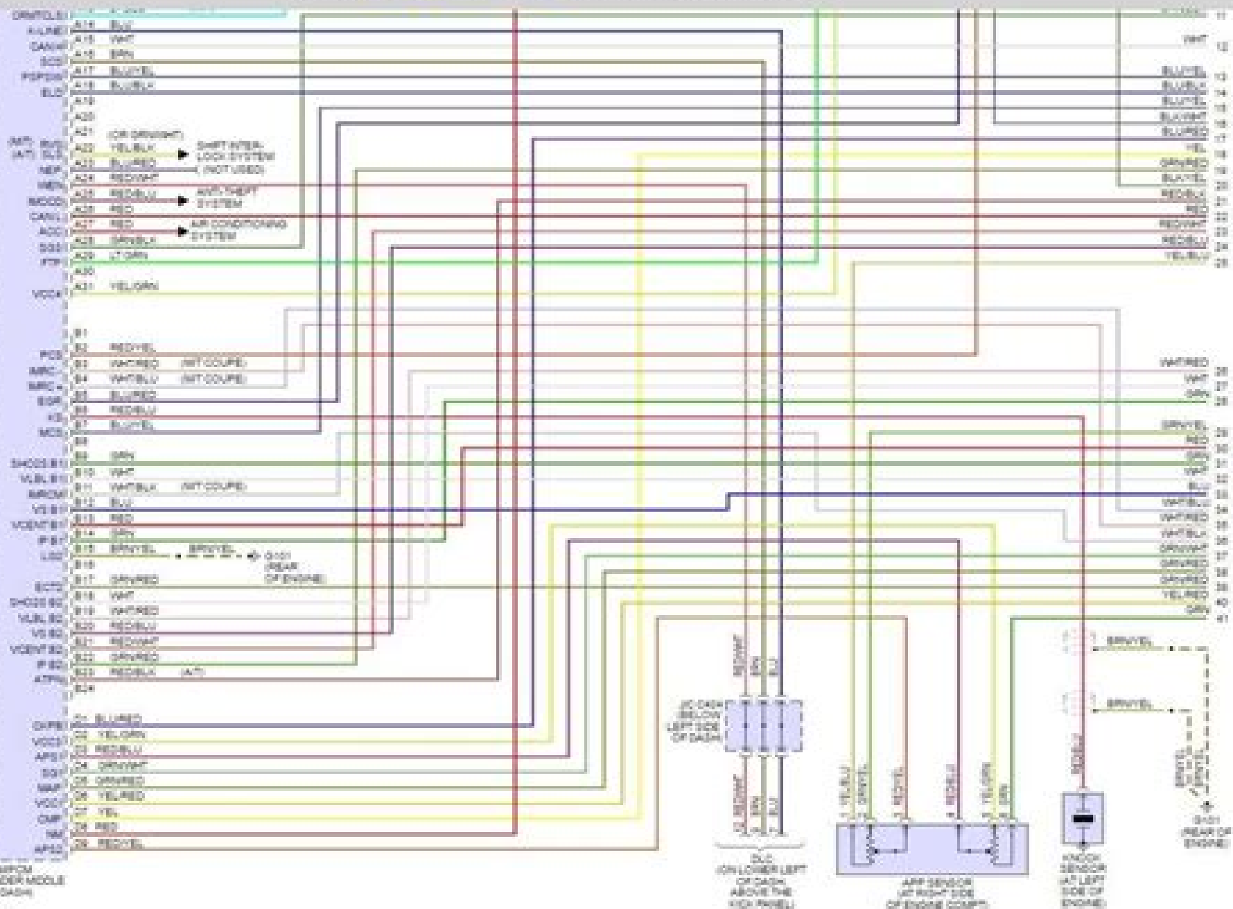
Fig 1: 3.0L Engine Performance Circuit, Except Hybrid (1 of 5)
