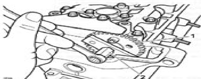
1. Exhaust camshaft 2. Tool T3880102
