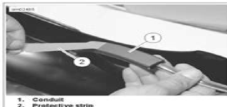
Figure 2-117. Removing Protective Strip from Conduit
