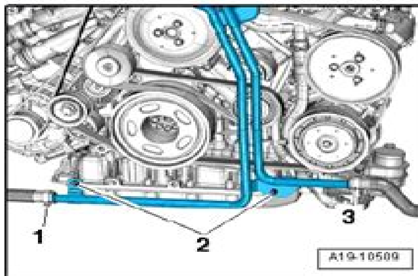
Fig 8: Identifying Hose Clamps -1 And 3- &amp; Left Front Coolant Hose
