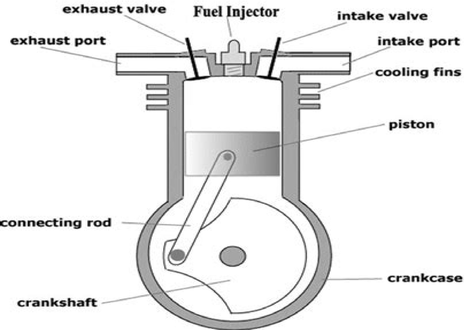
4 STROKE DIESEL ENGINE
