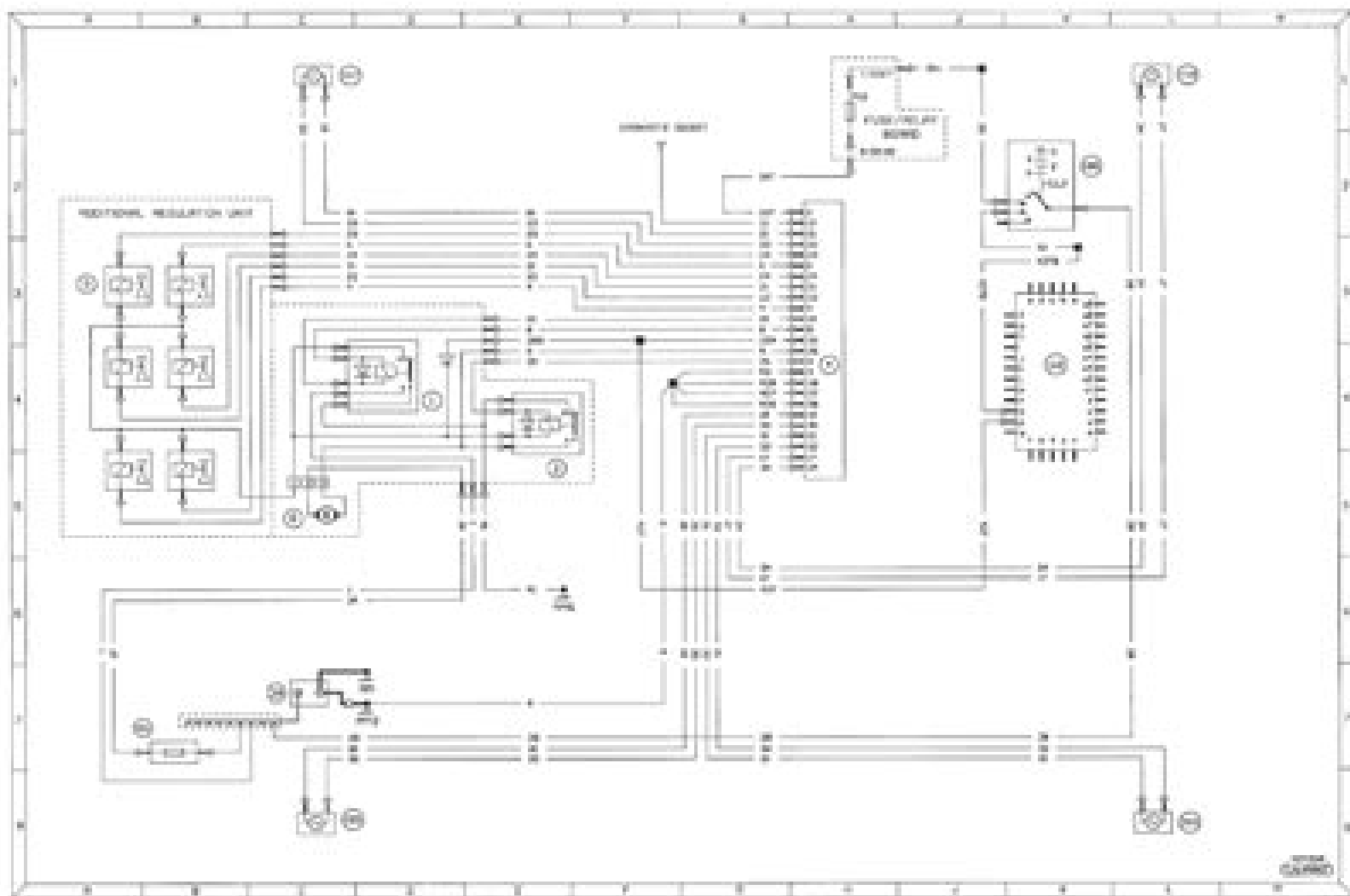
Diagram 4a : Optional anti-lock braking system - early models
