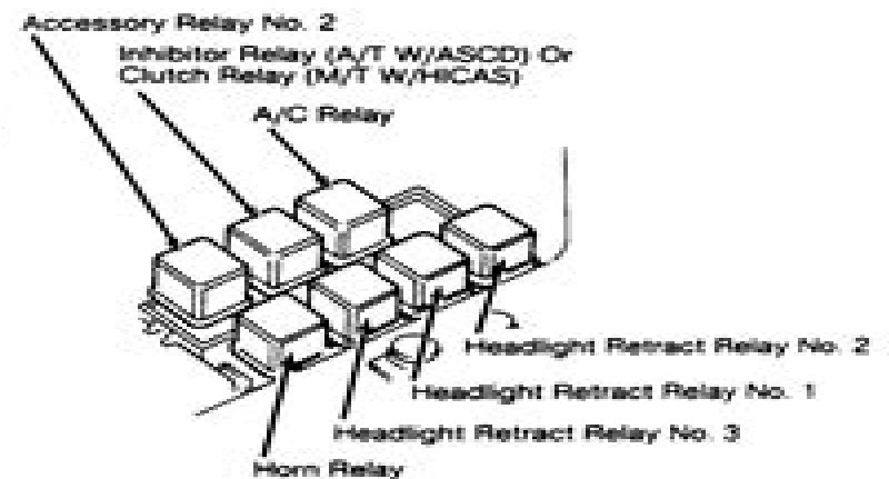
RELAY BOX
