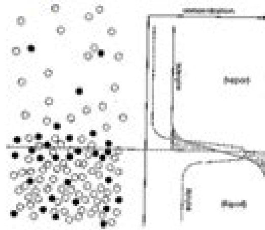
Figure 4.1. Concentration of solute and solvent molecules in the region of the interface.
