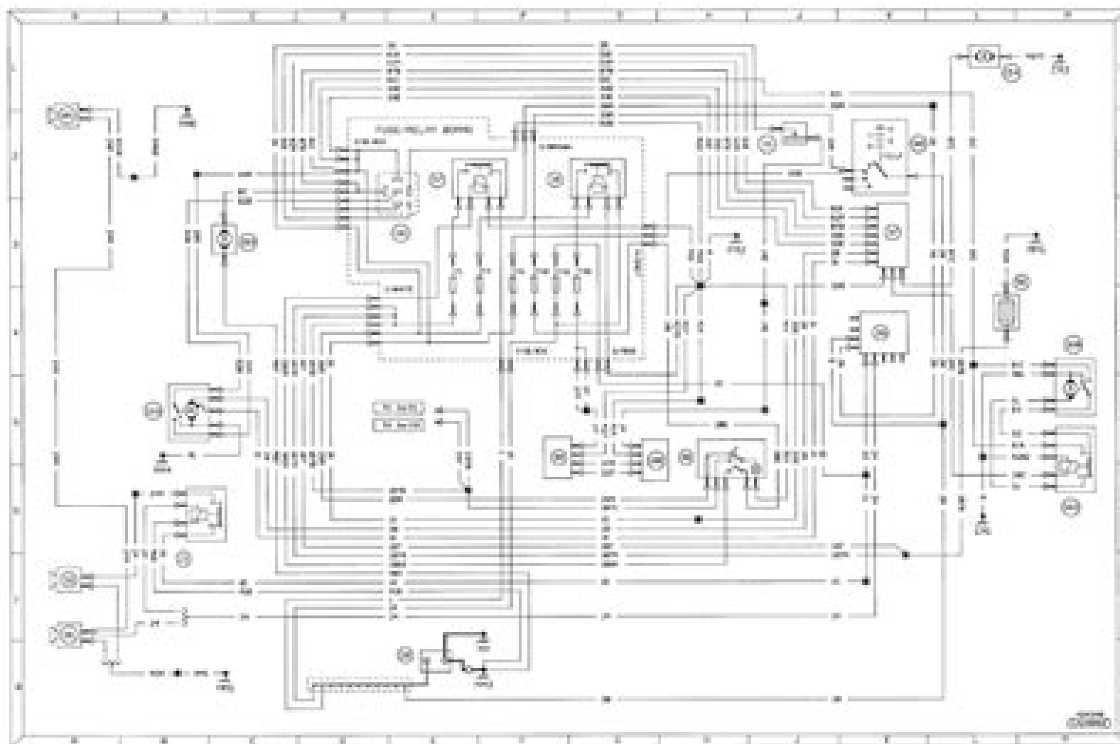
Diagram 3 : Typical auxiliary circuits (wash/wipe, horn, heater blower and heated rear window) - early models
