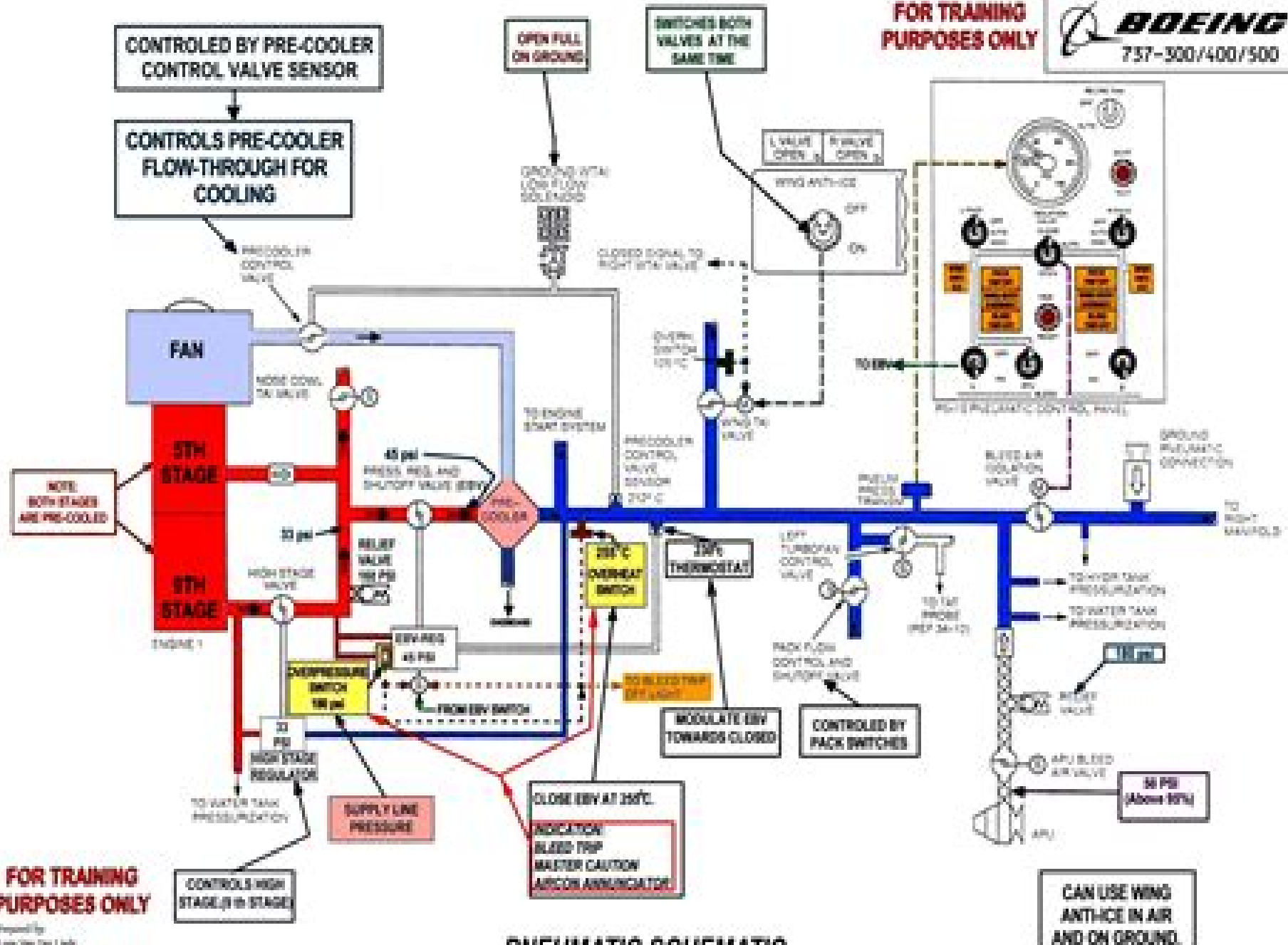
PNEUMATIC SCHEMATIC
