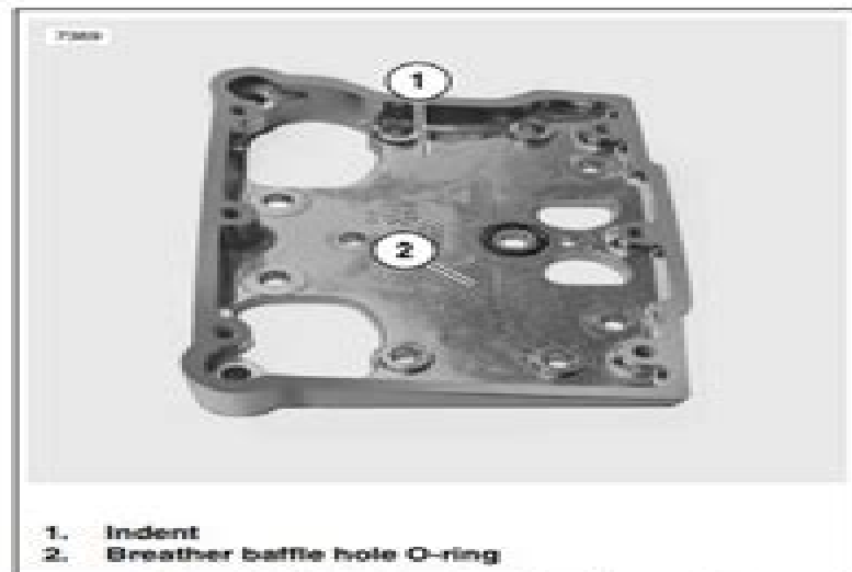
Figure 3-42. Rocker Housing Alignment
