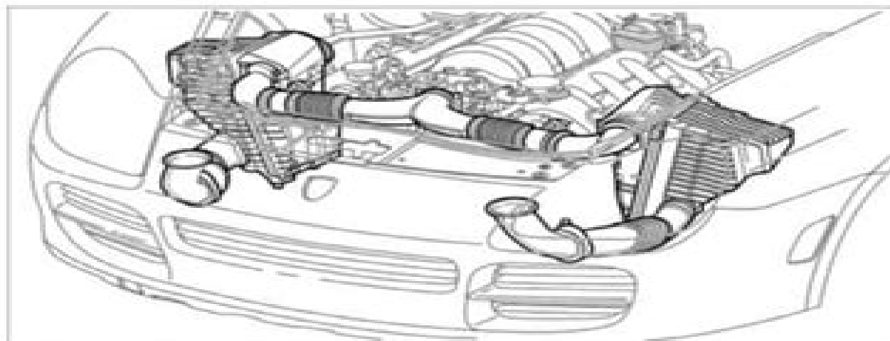
Fig. 1: Air guide for V8 S
