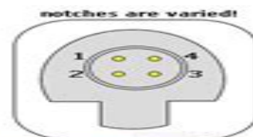
4 pin Head Unit LVDS shaped connector
