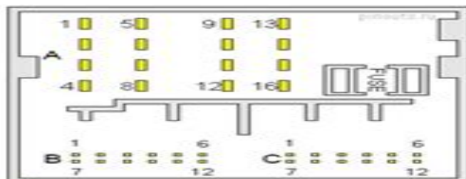
40 (16+12+12) pin QuadLock Fakra Head Unit / Car Stereo connector
