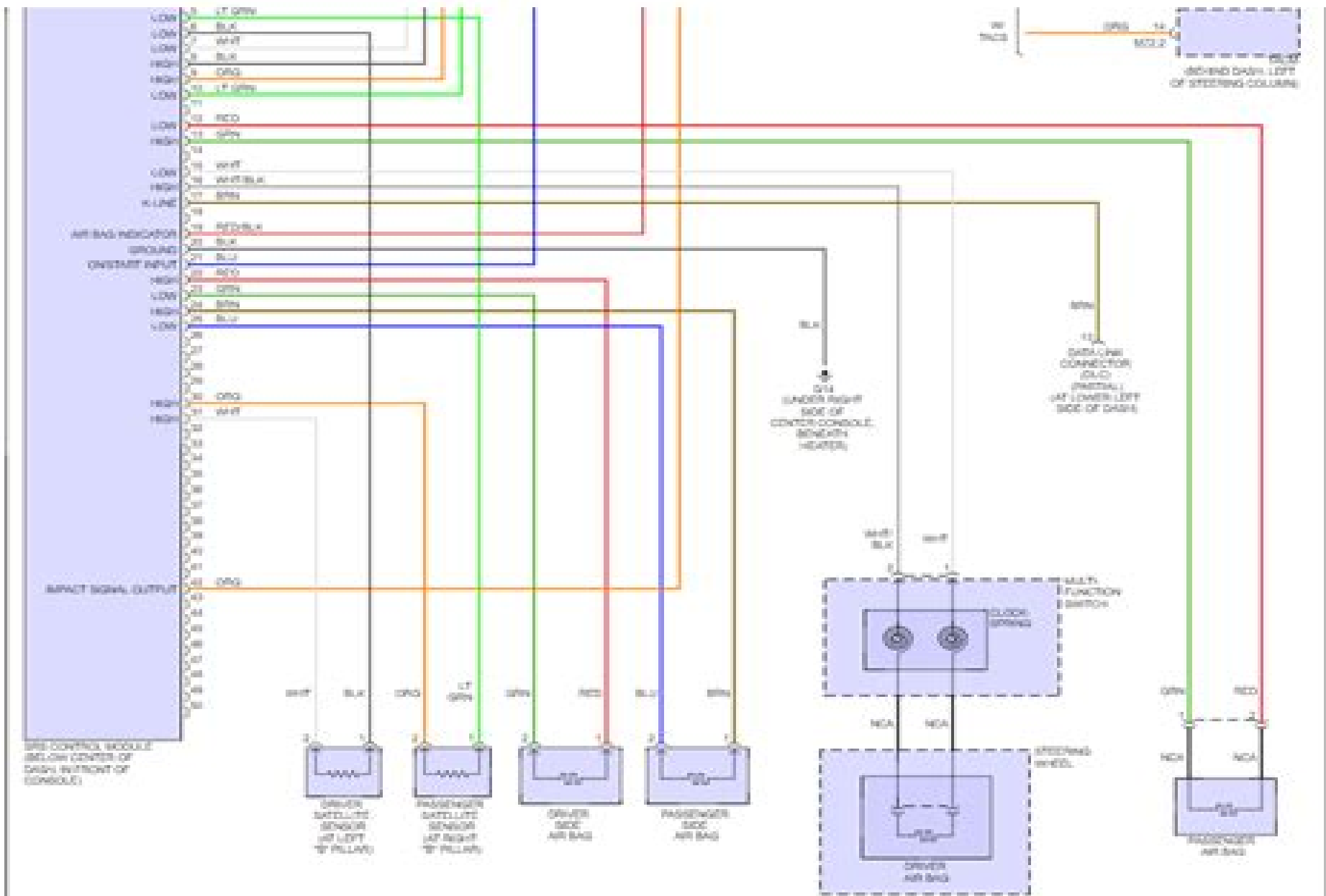
Fig 1: Supplemental Restraints Circuit, Base
