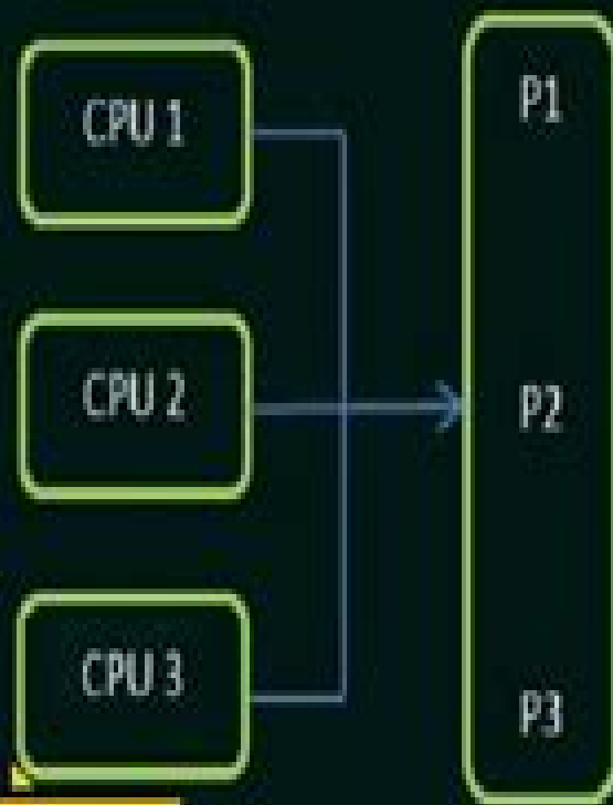
Symmetric Multiprocessing
