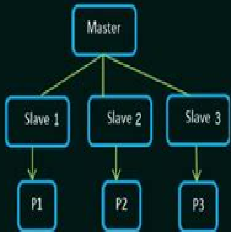
Asymmetric Multiprocessing
