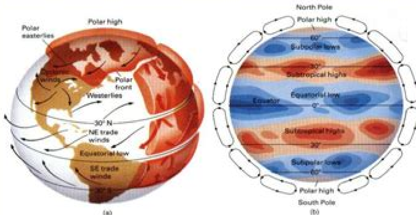
Two models of global wind patterns as predicted by the three-cell theory. (a) An artist's rendition showing the three cells and the directions of surface winds. (b) High and low pressure belts with the major convection currents shown on the edges of the sphere.
