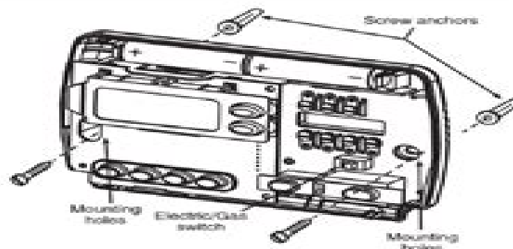
Figure 1. Thermostat Base
