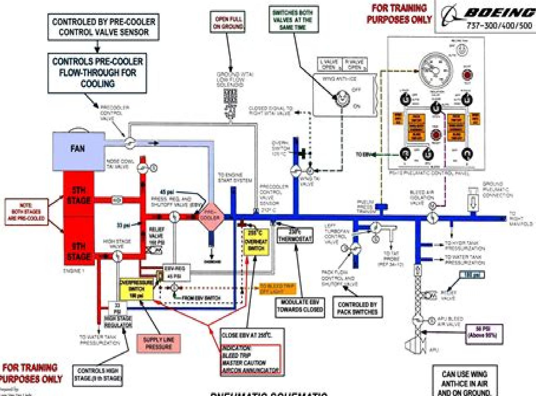
PNEUMATIC SCHEMATIC
