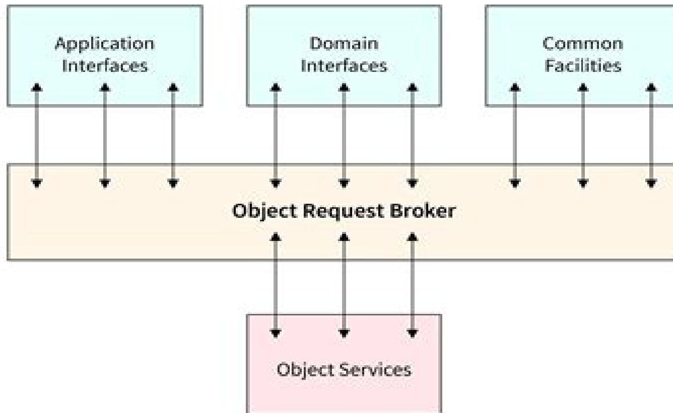
OMG Reference Model Architecture
